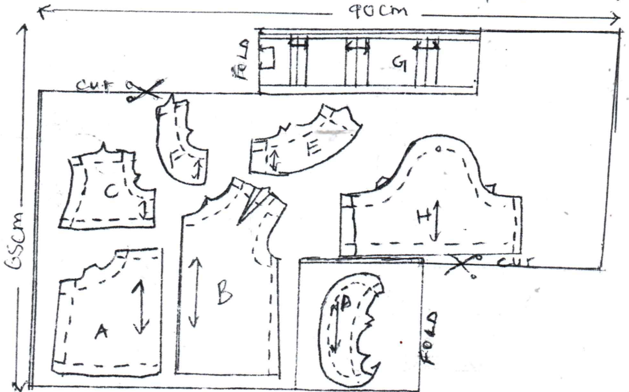
PATTERN LAYOUT (NOT DRAWN TO SCALE)
